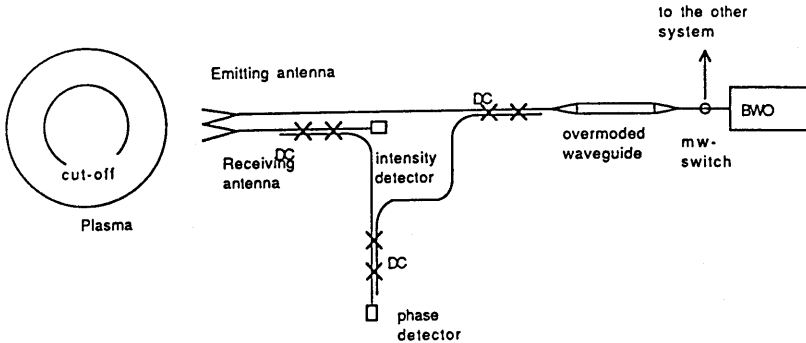
fig. 1 Principle of the reflectometer
