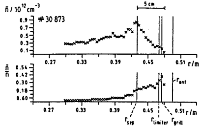
fig. 7 Absolute and relative electron density fluctuations as calculated from the data shown in fig. 5
