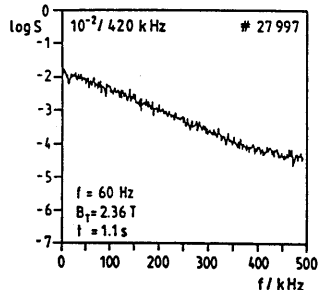
fig. 3 A typical power spectrum of the reflected intensity (fixed frequency launched)
