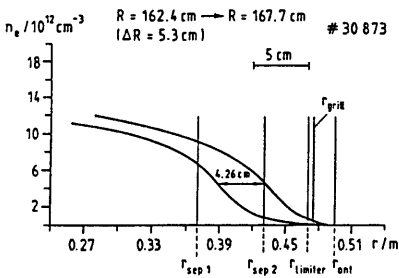
fig. 6 Density profiles measured in two stationary plasma phases in one shot, where the plasma has been moved horizontally 5.3 cm ( B = 2.8T , I_p = 420kA , n_e = 1.3 \times 10^{13}/cm^3 )
