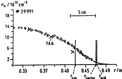
fig. 8 Comparison of the density profile measured with the reflectometer to the densities obtained with outermost channels of the Thomson scattering system (YAG). ( B = 2.8T , I_p = 320kA , n_e = 2.0 \times 10^{13}/cm^3 )
