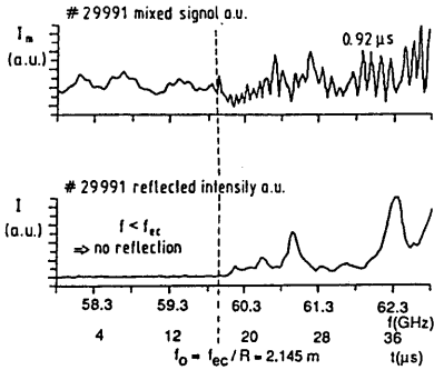
fig. 4 Raw data in sweep operation; upper tr.: mixed signal containing the phase information; lower tr.: intensity of the reflected signal ( B = 2.8T , I_p = 320kA , n_e = 2.0 \times 10^{13}/cm^3 )
