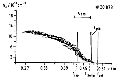
fig. 5 momentary profiles from 35 sweeps in a stationary plasma phase, superimposed (same plasma phase as in fig. 6, R = 167.7 cm) ( B = 2.8T , I_p = 420kA , n_e = 1.3 \times 10^{13}/cm^3 )
