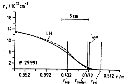
fig. 9. Profile change measured during LH experiments ( B = 2.8T , I_p = 320kA , n_e = 2.0 \times 10^{13}/cm^3 , P_{LH} = 1.3MW )
