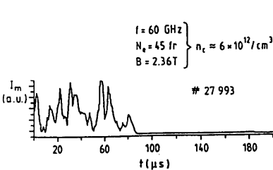
fig. 2 Intensity of the reflected signal from the plasma, fixed frequency; The launched signal has been chopped, so that the right part of the trace gives the baseline.
